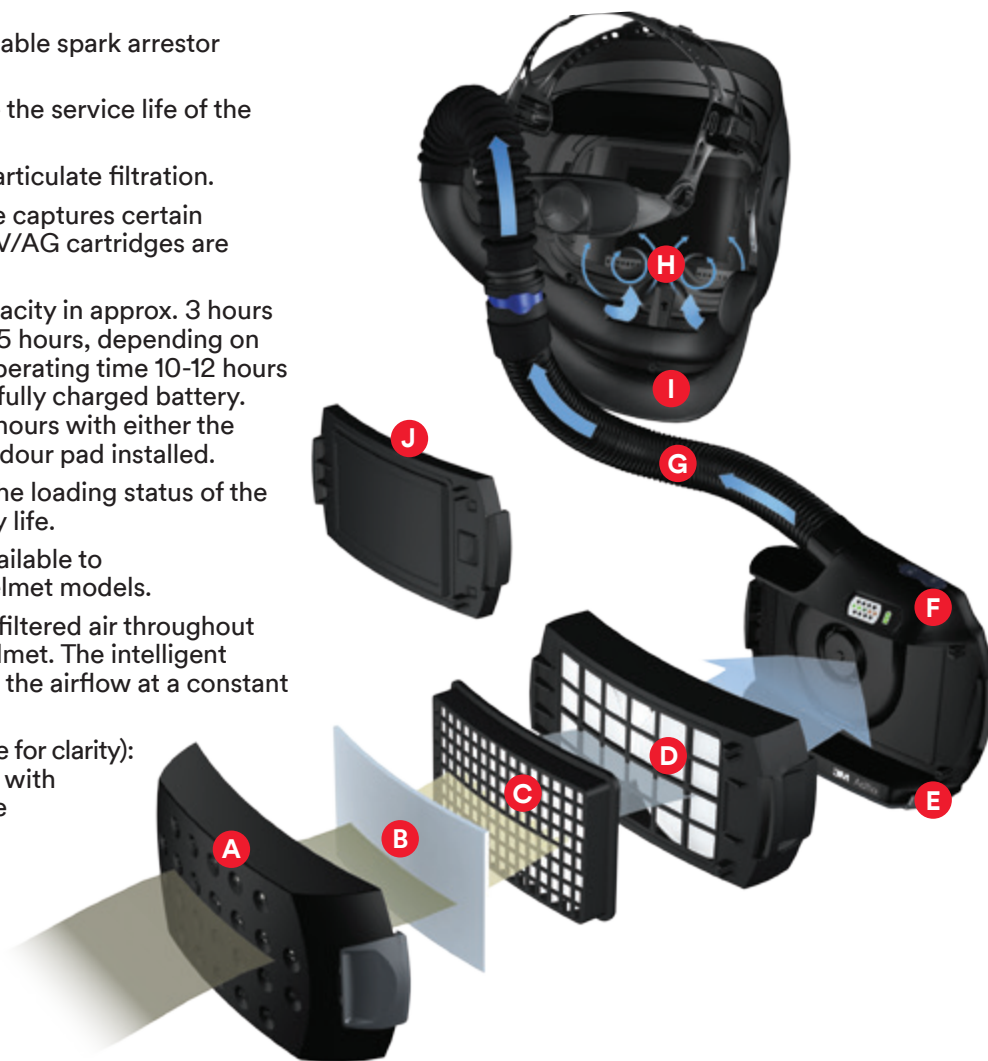
Shown here: 3M™ Adflo™ Powered Air Purifying Respirator with 3M™ Speedglas™ Welding Helmet 9100 FX-Air.
